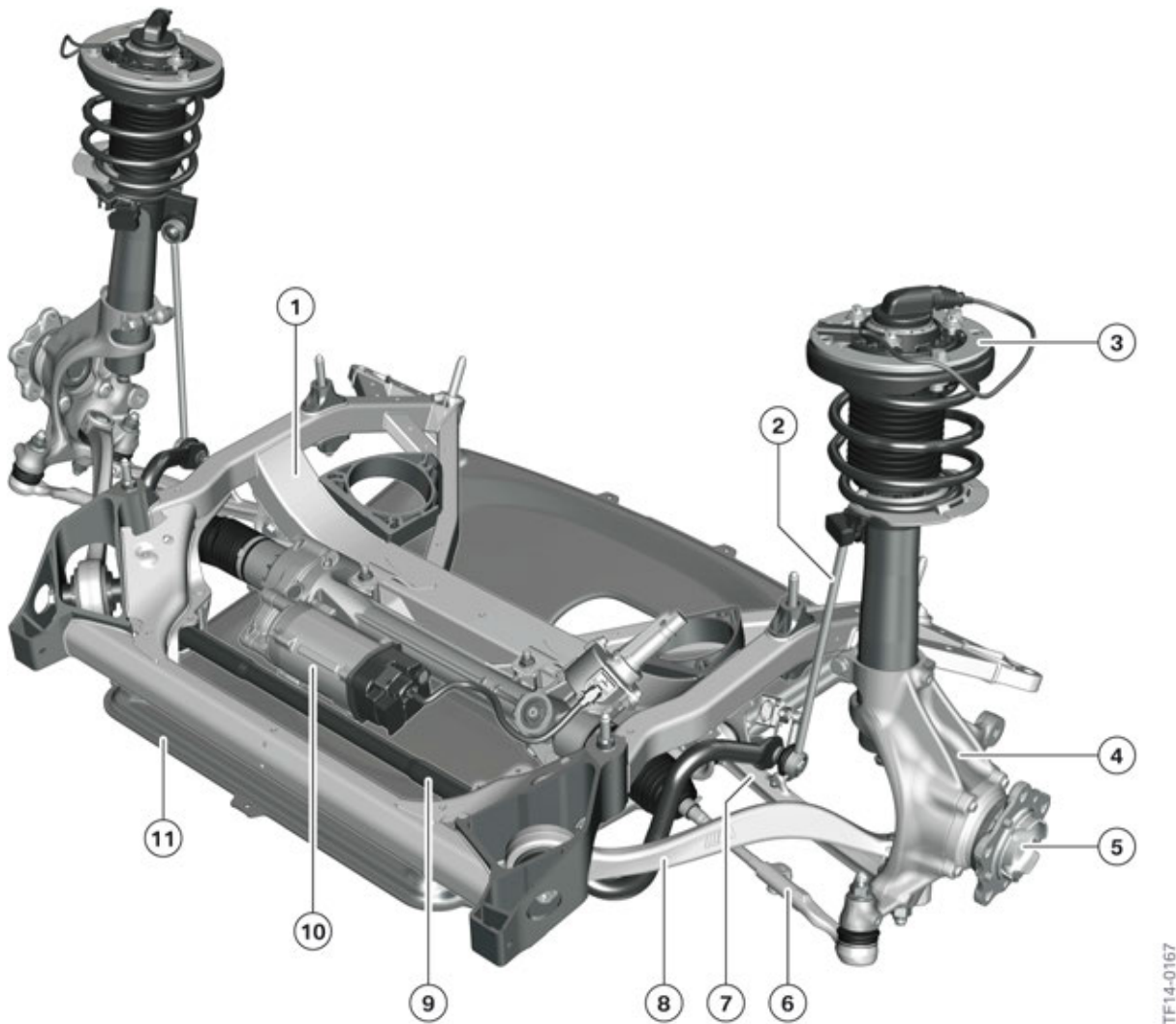
F80/F82 two-joint spring strut front axle
